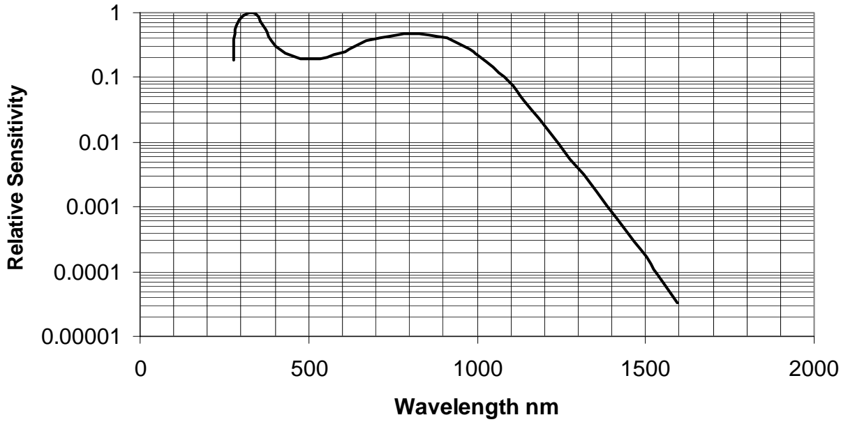
Nominal Sensitivity for models 84530A. Tested to see 1350 nm light from a 400 \mu W LED at 4.57 m, (15-ft.).
