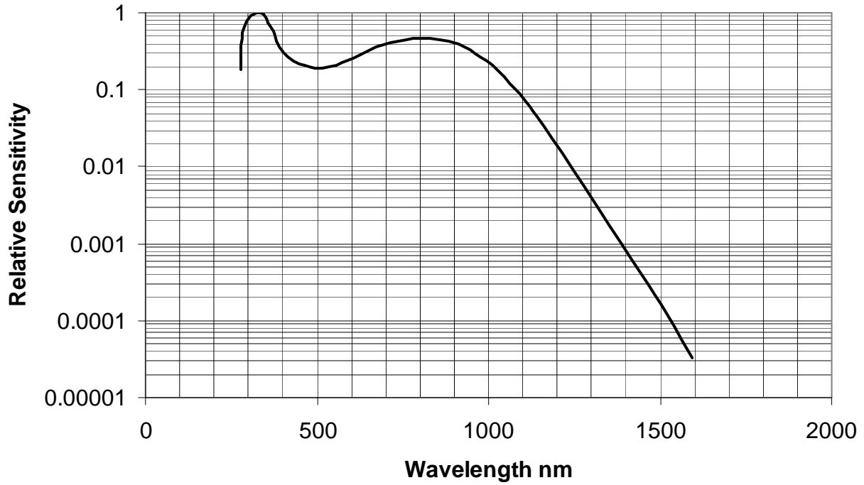
Nominal Sensitivity for models 85050. Tested to see 1550 nm light from a 350 \mu W LED at 2.44 m, (8-ft.).
