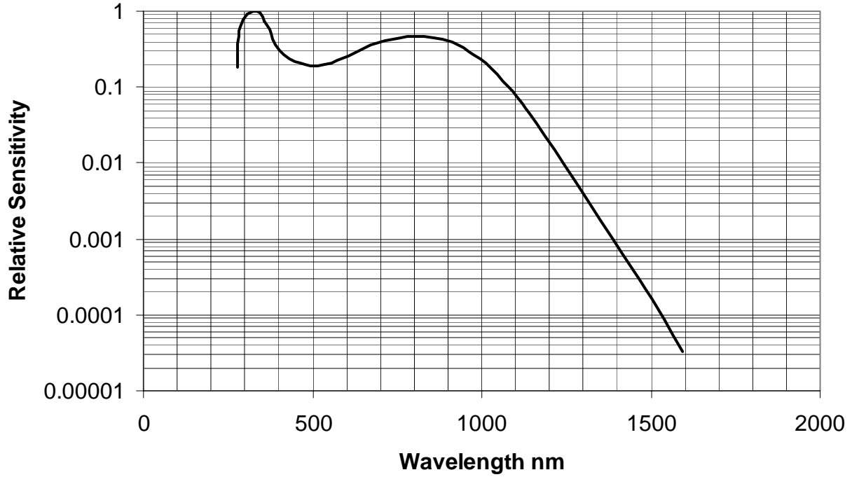
Nominal Sensitivity for models 85051A-5. Tested to see 1550 nm light from a 350 \mu W LED at 2.44 m, (8-ft.).
