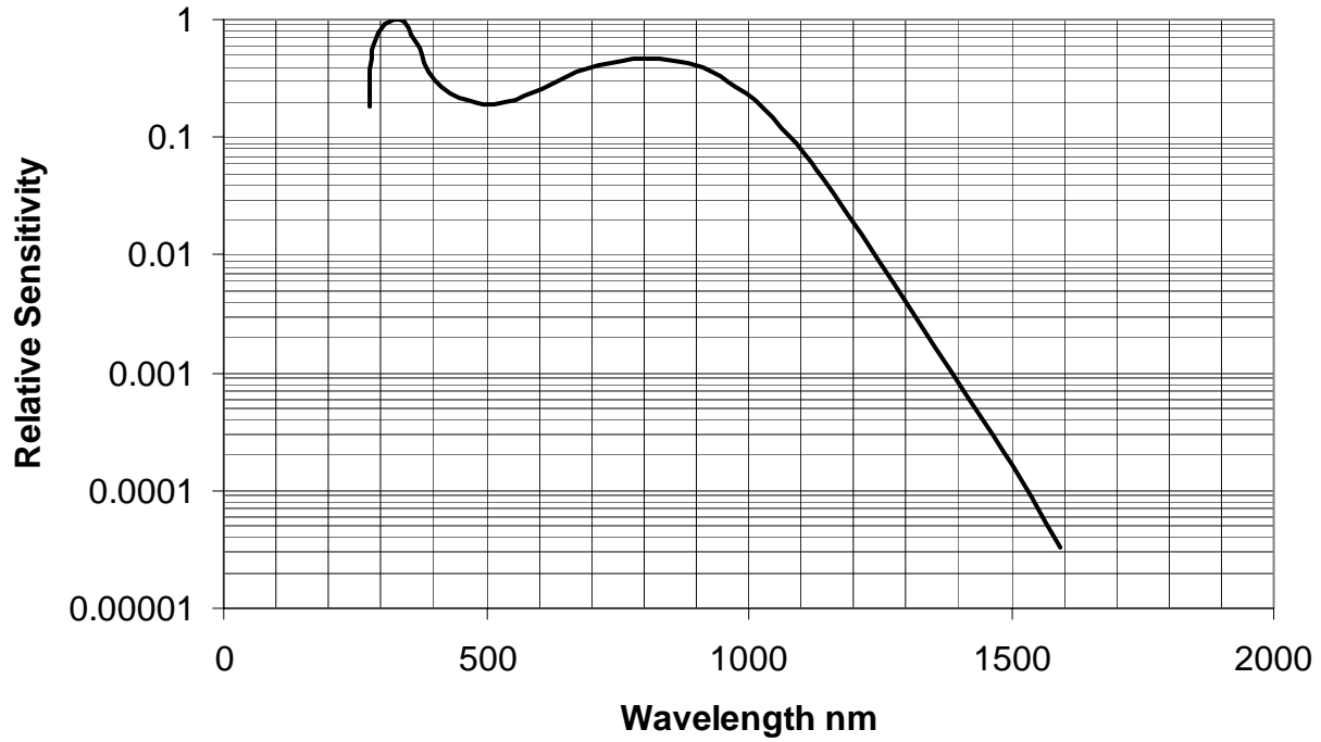
Nominal Sensitivity for models 85268 & 85268A. Tested to see 1350 nm light from a 400 \mu W LED at 4.57 m, (15-ft.).
